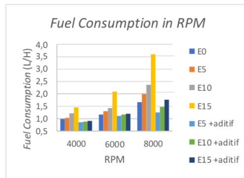
Figure 5. Fuel Consumption in RPM.
