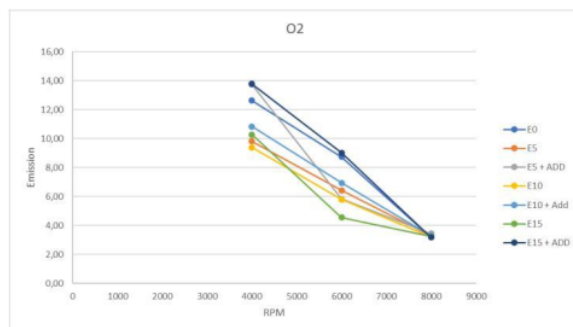
Figure 4. O 2 vs Engine Speed.
