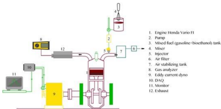
Figure 1. Experimental Set up Engine.
