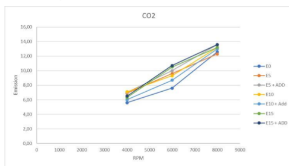
Figure 2. CO 2 vs Engine Speed.
