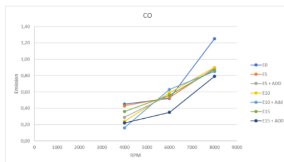
Figure 3. CO vs Engine Speed.
