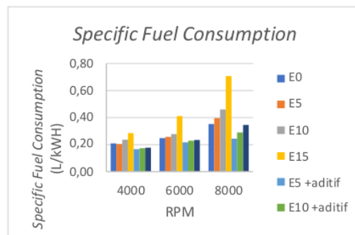
Figure 6. Specific Fuel Consumption.
