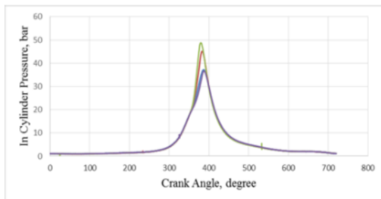
9 FIGURE 2. In-Cylinder Pressure vs. Crank Angle (E5)
