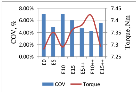
FIGURE 5. COV vs. Torque
