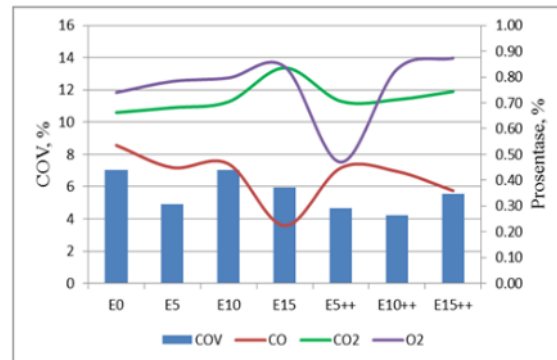
FIGURE 6. COV vs. CO, CO 2 , & O 2
