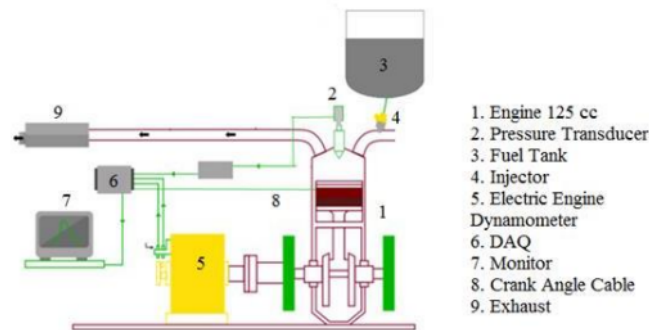
FIGURE 1. Experimental Set up Engine
