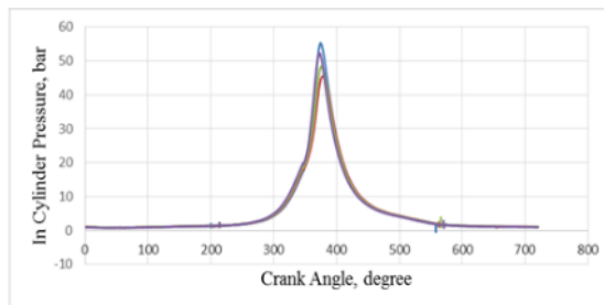
FIGURE 3. In-Cylinder Pressure vs. Crank Angle (E10++)
