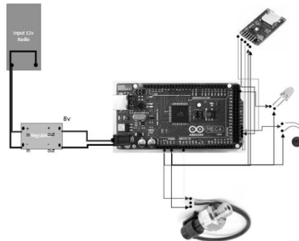
Gambar 4. Clogging Detector
